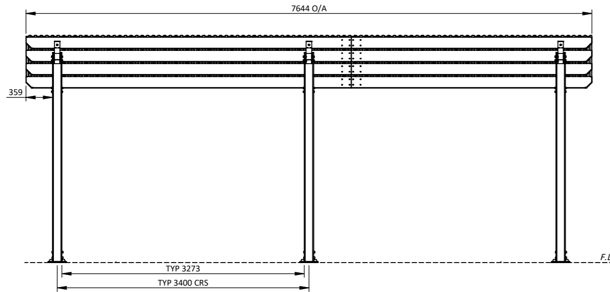
FRONT VIEW 1:50
