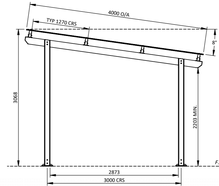
SIDE VIEW 1:50
