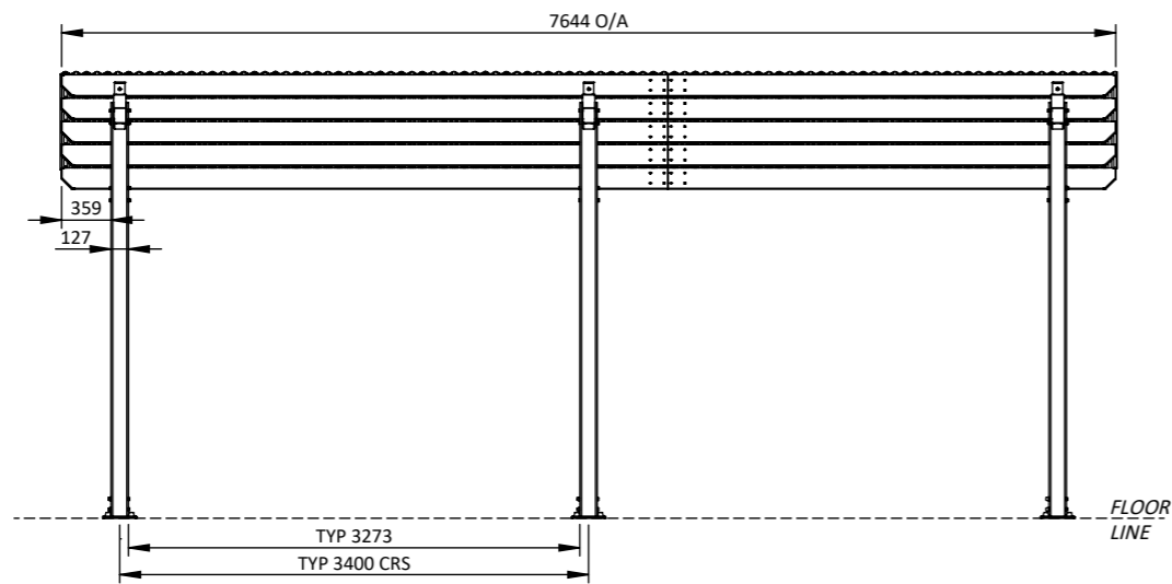
FRONT VIEW 1:60
