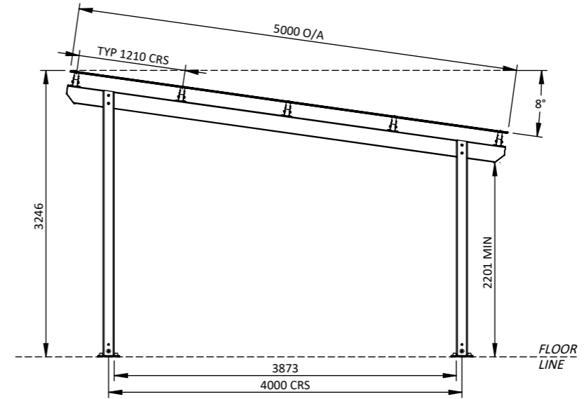
SIDE VIEW 1:60
