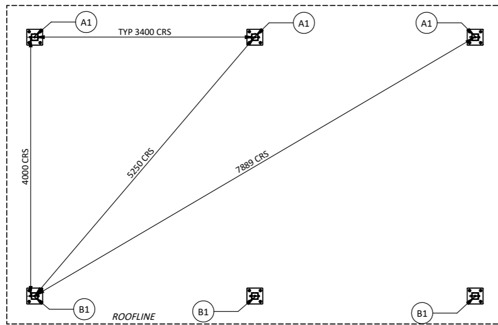
FOUNDATION PLAN 1:60
