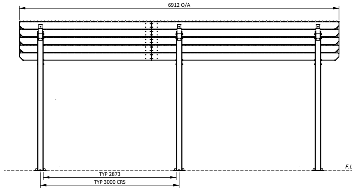
FRONT VIEW 1:50
