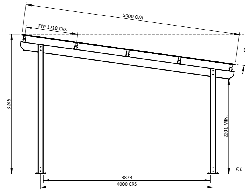
SIDE VIEW 1:50
