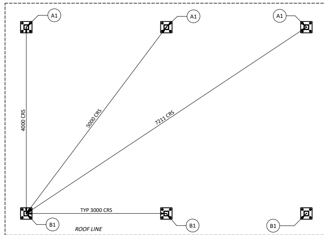
FOUNDATION PLAN 1:50
