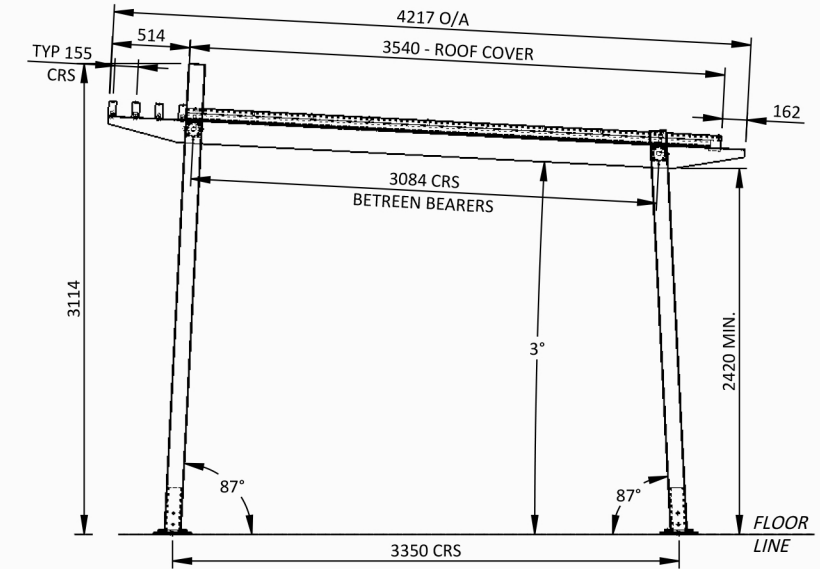
SIDE VIEW 1:50
