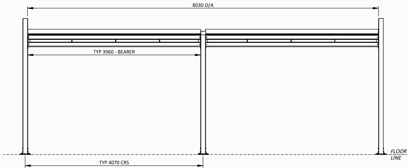
FRONT VIEW 1:50
