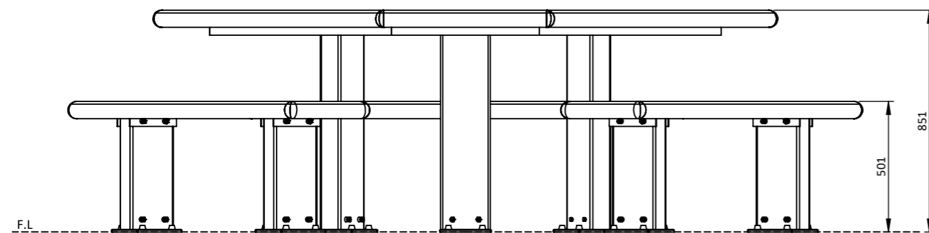
FRONT VIEW 1:20
