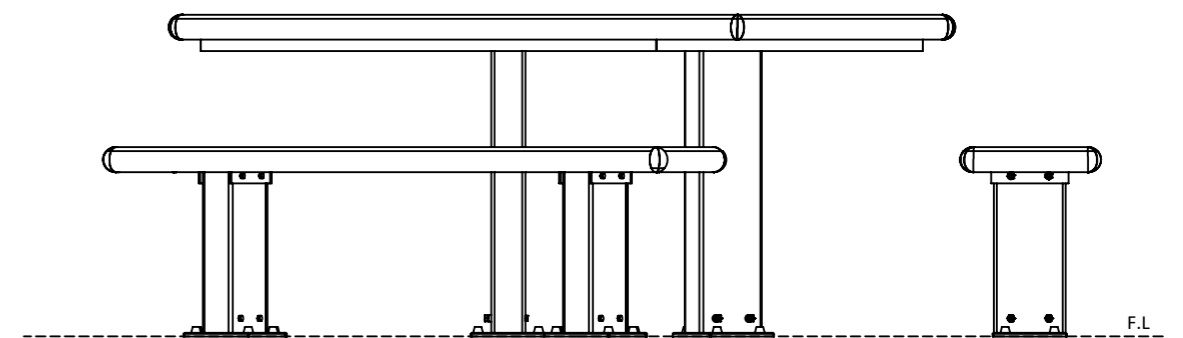
FRONT VIEW 1:20
