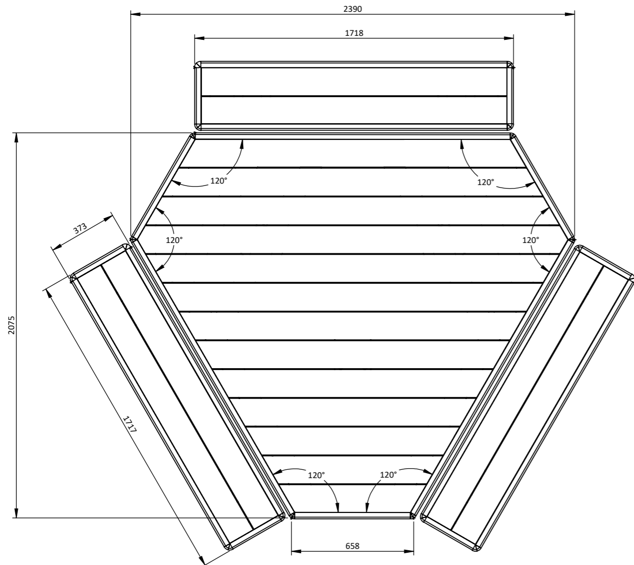
TOP VIEW 1:20
