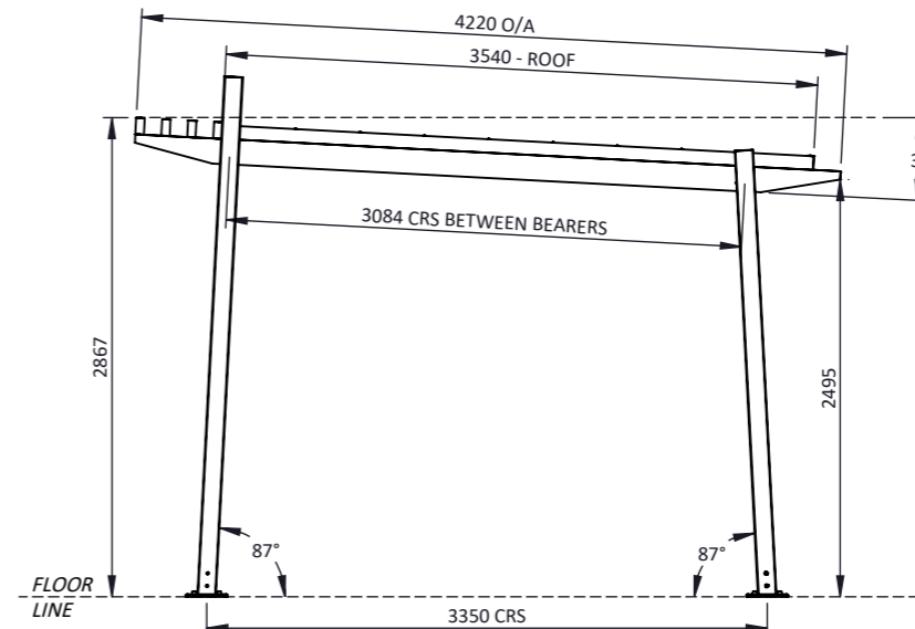
SIDE VIEW 1:50
