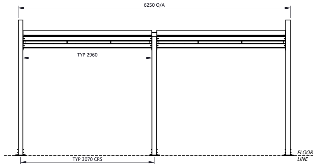
FRONT VIEW 1:50
