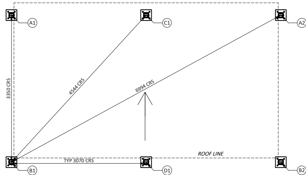
FOUNDATION PLAN 1:50
