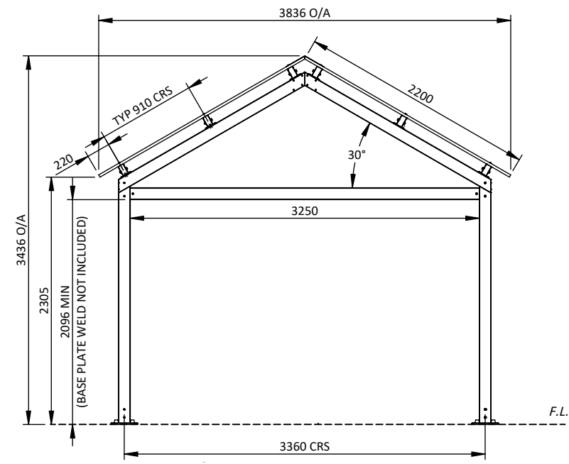
SIDE VIEW 1:50
