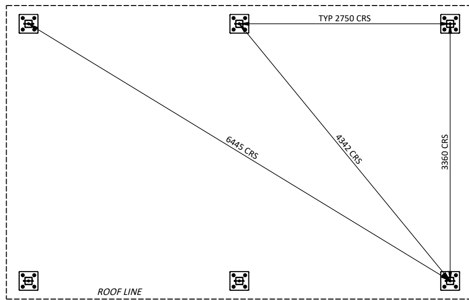
FOUNDATION PLAN 1:50
