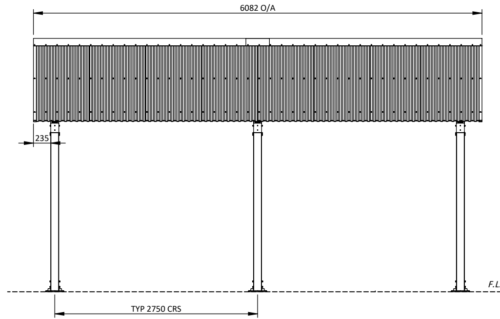
FRONT VIEW 1:50
