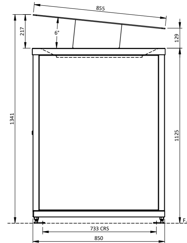
SIDE ELEVATION
