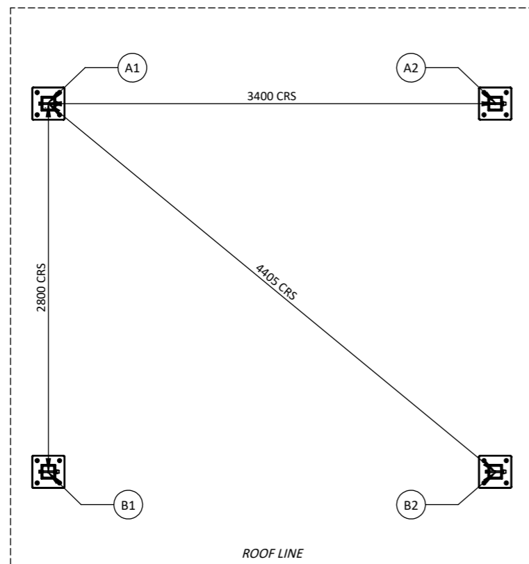
FOUNDATION PLAN 1:40
