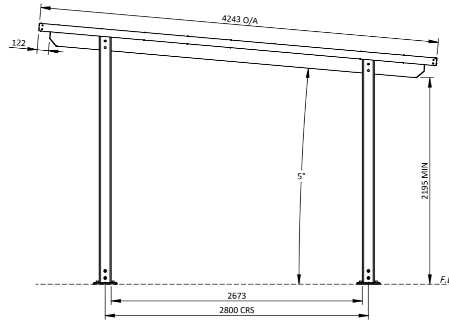
SIDE VIEW 1:40
