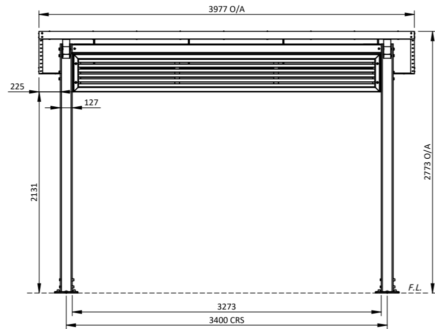
FRONT VIEW 1:40
